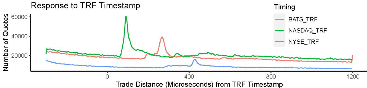
Panel B: Exchange quoting activity measured against NASDAQ TRF Timestamp.
